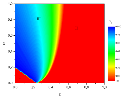
FIGURE 12. Contour graph of the critical value \gamma_c with respect to \varepsilon and \alpha , where k = 1 , \beta = 0.14 , \delta_E = \delta_I = \delta_H = 0.1 and \Delta_{in} = \Delta_{out} = 0 . The contour graph represents different values of \gamma_c .
