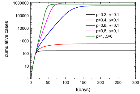
FIGURE 13. Evolution of the SEIHR model when intervention measures are involved, where q = 1 , k = 1 , \beta = 0.14 , \gamma = 1 , \delta_E = \delta_I = \delta_H = 0.1 , \varepsilon = 0.25 , and \alpha = 0.5 . The black solid line, red solid line, blue solid line and pink solid line represent the cumulative number of cases for different levels of intervention without closing the border. The green solid line represents the cumulative number of cases without intervention, but with border closed.
