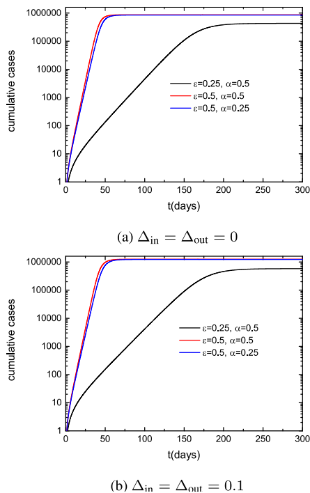
FIGURE 5. Evolution of the SEIHR model, where q = 1, k = 1, \beta = 0.14, \gamma = 1, \delta_E = \delta_I = \delta_H = 0.1 . The black solid line, red solid line and blue solid line represent the cumulative number of cases for different transmission rates.
