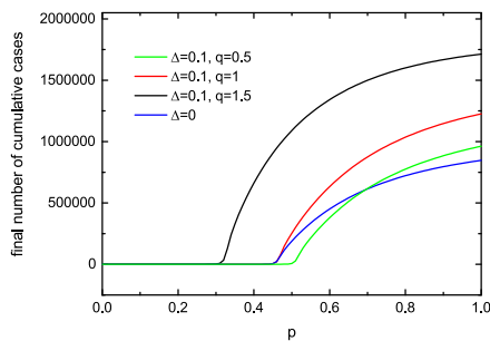
FIGURE 7. Relationship between the final number of cumulative case and p , where k = 1, \beta = 0.14, \gamma = 1, \delta_E = \delta_I = \delta_H = 0.1, \epsilon = 0.25 , and \alpha = 0.5 . The red solid line represent the final number of cumulative cases for different levels of intervention with or without closing the border.
