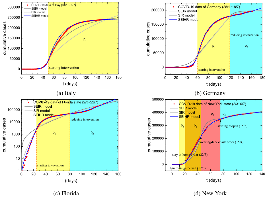
FIGURE 10. The SEIHR, SIR, SEIR model fits with the COVID-19 data in four different regions. The solid lines and the red dots represent simulation results and real data, respectively.
