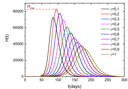
FIGURE 4. Evolution of the SEIHR model, with k = 1, \varepsilon = 0.25, \alpha = 0.5, \beta = 0.14, \delta_E = \delta_I = \delta_H = 0.1 and \Delta_{in} = \Delta_{out} = 0 . The colored solid lines represent H(t) for different values of \gamma .
