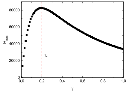
FIGURE 11. Relationship between H_{max} and \gamma , where k = 1 , \varepsilon = 0.25 , \alpha = 0.5 , \beta = 0.14 , \delta_E = \delta_I = \delta_H = 0.1 and \Delta_{in} = \Delta_{out} = 0 . The black squares represent H_{max} for different values of \gamma .
